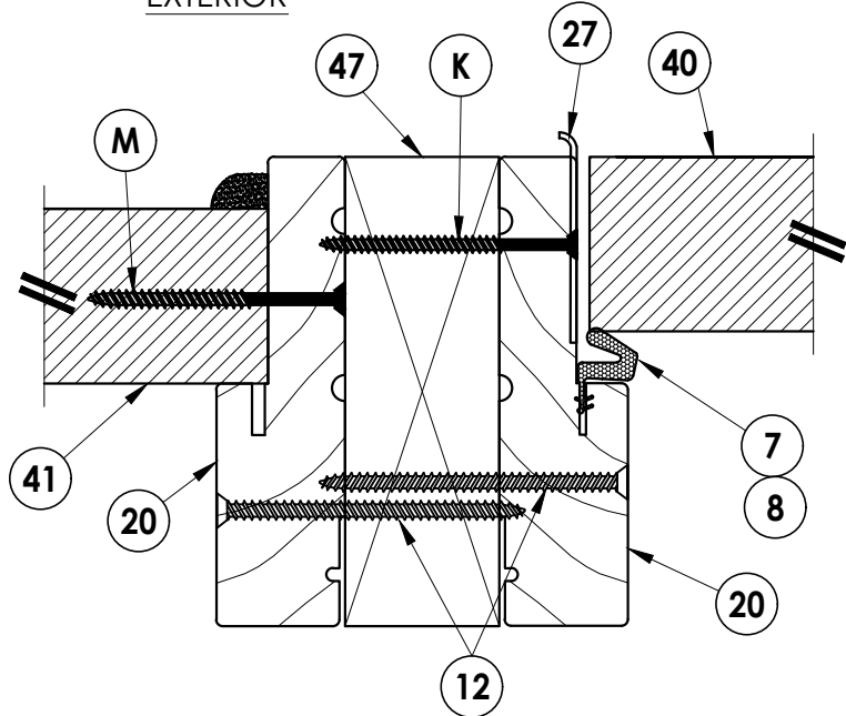
4 HORIZONTAL CROSS SECTION 4 Outswing strike jamb @ sidelite jamb
