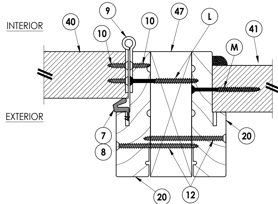
3 HORIZONTAL CROSS SECTION 4 Inswing hinge jamb @ sidelite jamb
