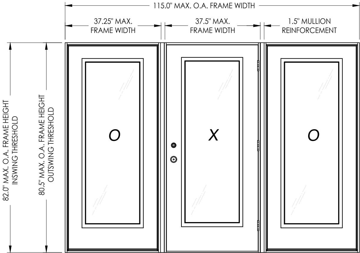
GLAZED SINGLE DOOR W/SIDELITES
