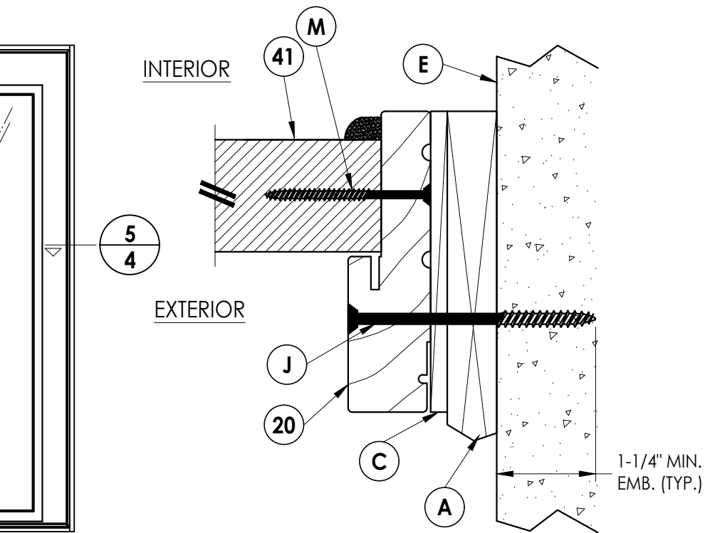
5 HORIZONTAL CROSS SECTION 4 Shown w/1X sub-buck
